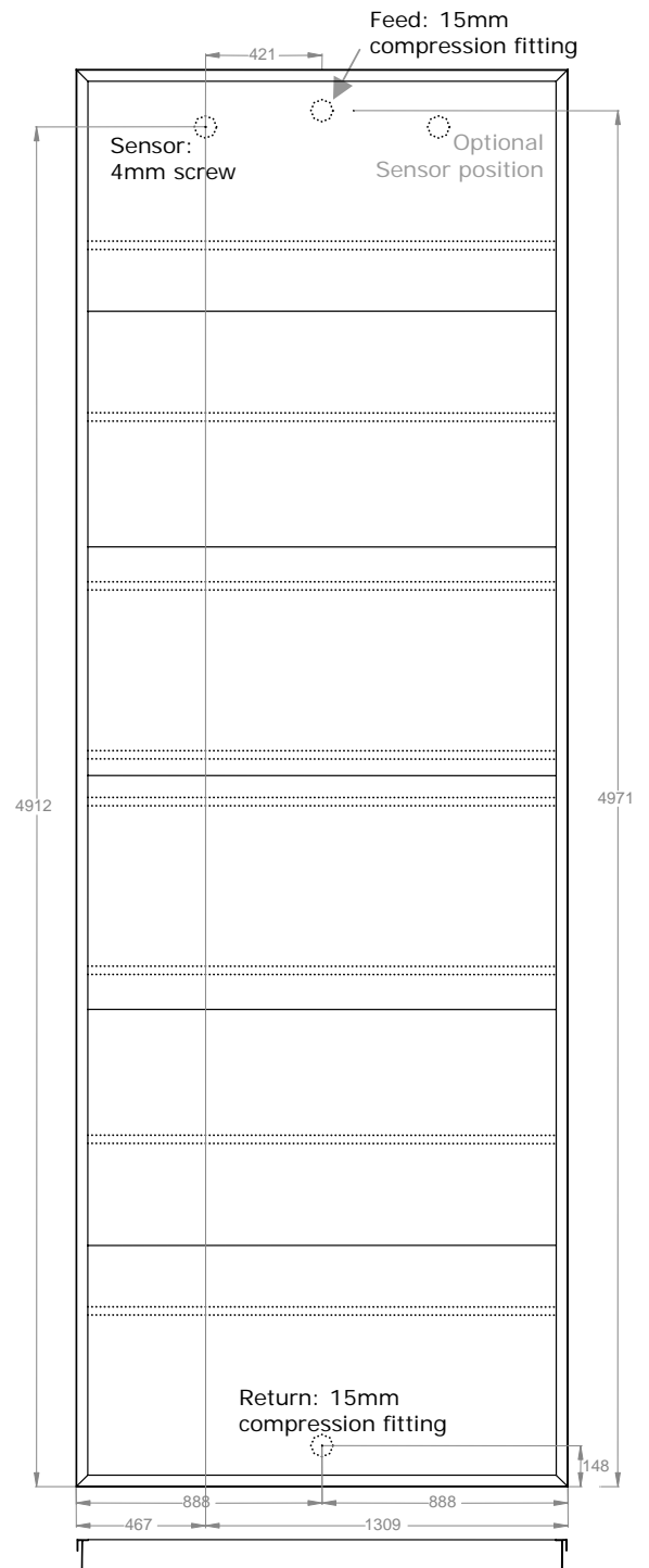
Connections (Viewed from glass front)
