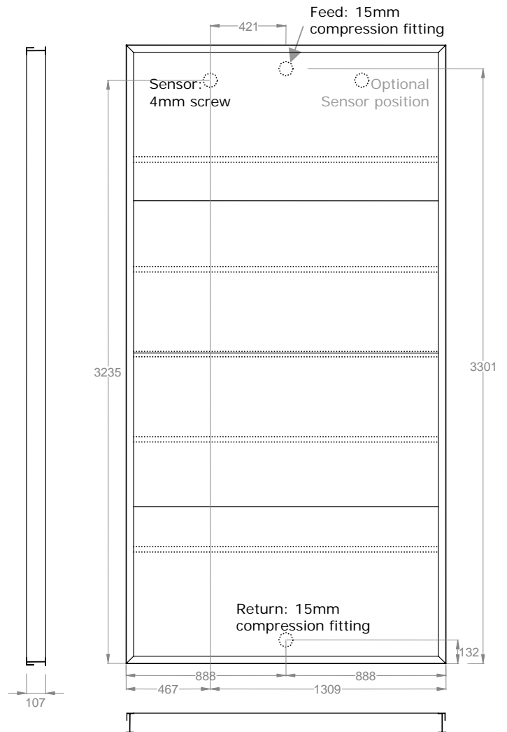
Connections (Viewed from glass front)
